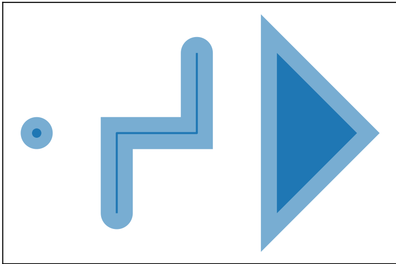
s.buffer(0.2, join_style=2)
