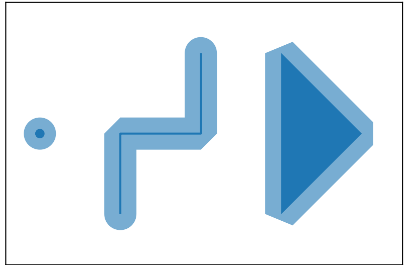
s.buffer(0.2, join_style=3)
