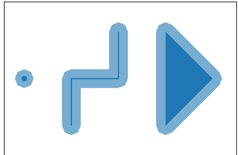
s.buffer(0.2, resolution=2)
