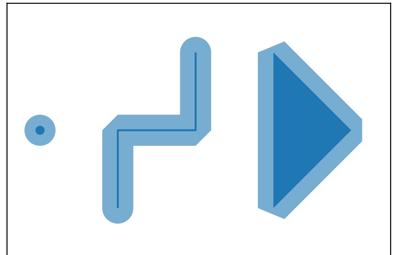
s.buffer(0.2, join_style=3)
