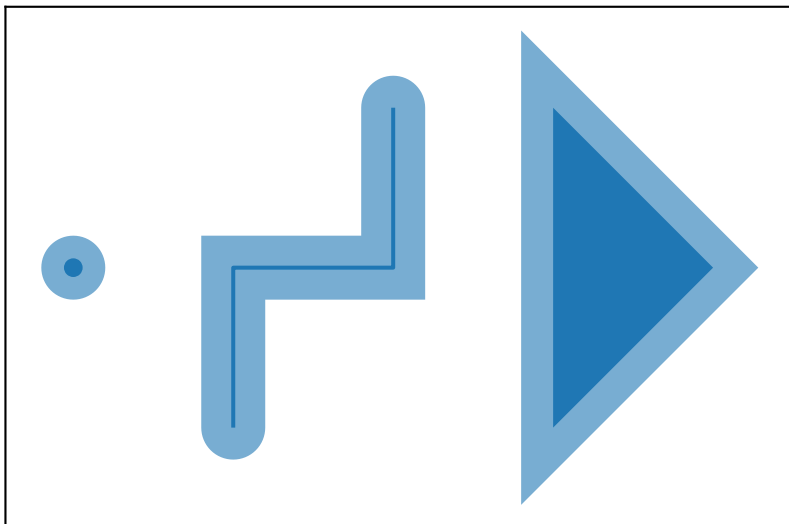
s.buffer(0.2, join_style=2)
