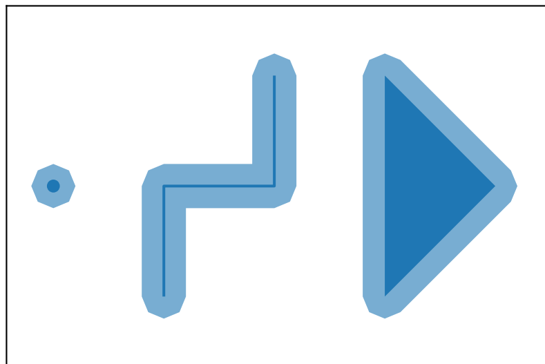
s.buffer(0.2, resolution=2)
