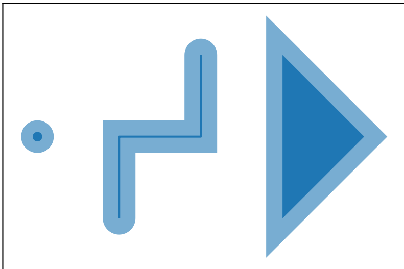
s.buffer(0.2, join_style="mitre")
