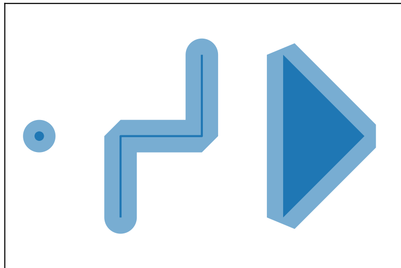
s.buffer(0.2, join_style="bevel")
