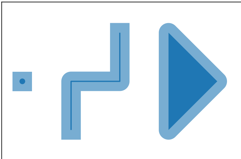
s.buffer(0.2, cap_style="square")
